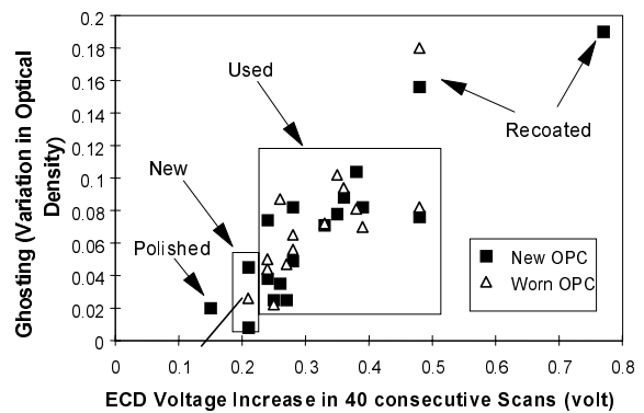
Figure 6. Correlation between Variation in Optical Density with ECD Voltage Increase in Charge Accumulation Test.
