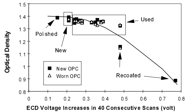
Figure 5. Correlation between Optical Density in Solid Black Area with ECD Voltage Increase in Charge Accumulation Test.
