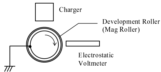
Figure 2. Schematic of Electrostatic Charge Decay Measurement
