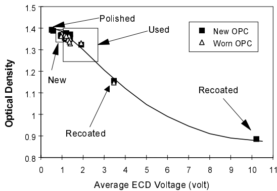
Figure 3. Correlation between Optical Density in Solid Black Area with Average Residual Voltage from ECD Mapping.
