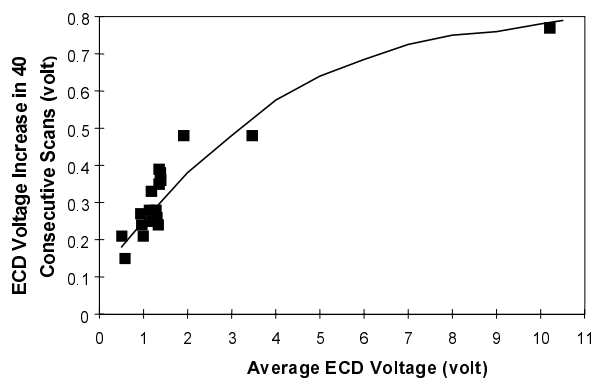
Figure 7. Correlation Between Charge Accumulation Test and Residual Voltage Map
