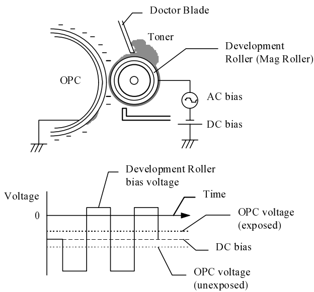
Figure 1. Developing an Image on the OPC in a Magnetic Monocomponent Development System
