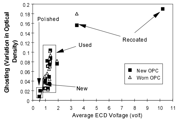
Figure 4. Correlation between Variation in Optical Density with Average Residual Voltage from ECD Mapping.
