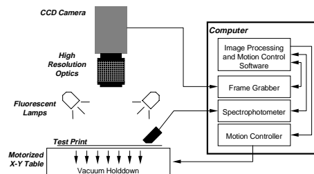
Figure 1 Print Quality Analysis System Hardware Architecture
